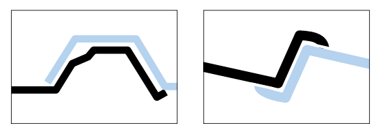
CORRECT LAP DETAIL FOR VARIOUS INFILL SHEET PROFILES
